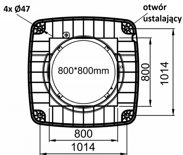
Wylot dolny "D"
